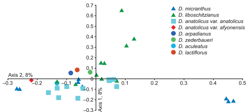
Fig. 3. PCoA plot of the first two coordinates of AFLP data from the studied accessions.
