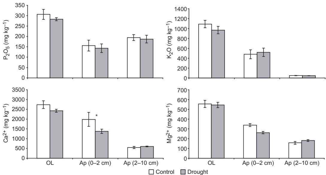
Fig. 4. Effect of drought on concentrations of P, K, Ca 2+ and Mg 2+ in organic layer (OL) and layers of mineral soil Ap (0–2 cm) and Ap (2–10 cm) in 2004 m. An asterisk (*) indicates a significant difference at p < 0.05 ( t -test).
