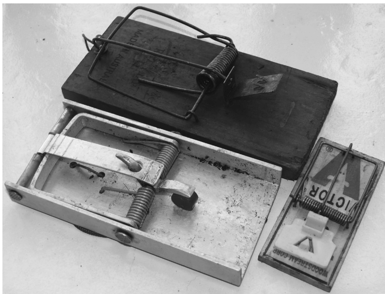
Fig. 1. Set prototype Ka Mate Medium Pro Trap (below left), Ezeset Supreme Rat Trap (upper left) and Victor Professional Mouse Trap (right).
