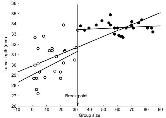
Fig. 2. Relationship between group size and larval length close to pupation time of experimental colonies. Solid line represent the Piecewise Linear Regression ( R = 0.91 , N = 50 , p < 0.001 ) and discontinuous lines represent linear regression ( R = 0.76 , N = 50 , p < 0.001 ). Differences between correlation coefficients: p < 0.05 .
