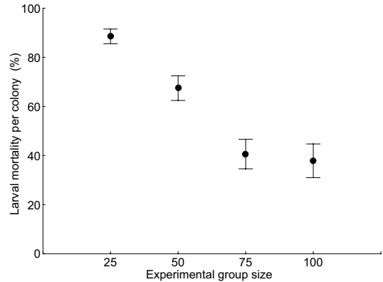
Fig. 3. The average percentage of larval mortality in the four group size treatments. Differences in the means were significant (ANOVA: F_{3,56} = 19.63 , p < 0.001 ).
