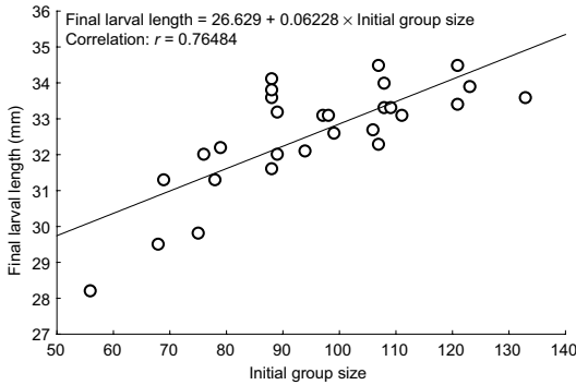
Fig. 1. Relationship between the initial group size and the final larval size in natural colonies. Test used was Spearman rank correlation. N = 28 .
