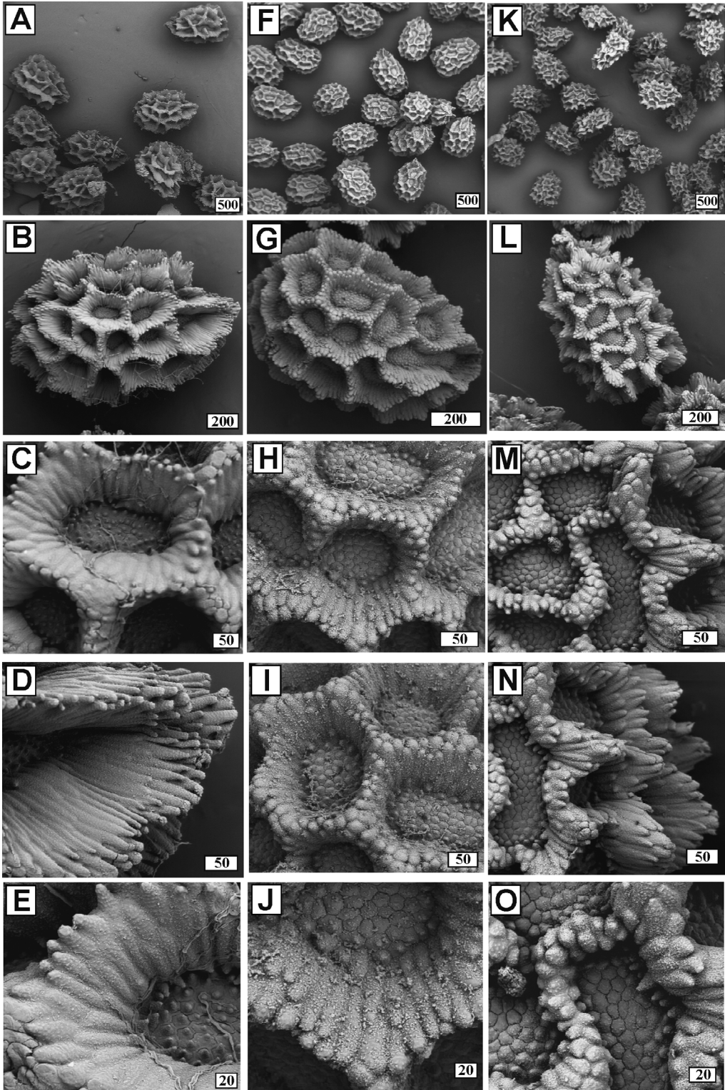
Fig. 7. SEM microphotographs showing types of ornamentation of Antirrhinum seeds. — A–E: A. braun-blanquetii . — F–J: A. meonanthum . — K–O: A. rothmaleri . Scale bars = \mu\text{m} .
