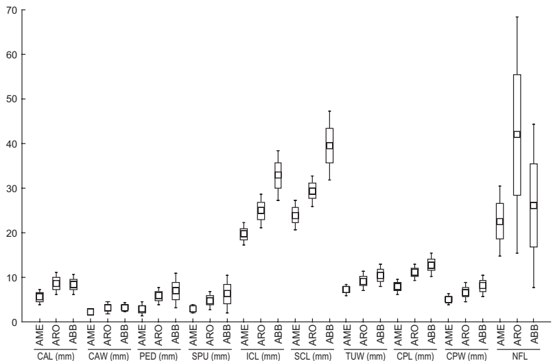
Fig. 6. Variation in selected morphological traits of A. meonanthum (AME), A. rothmaleri (ARO), and Antirrhinum braun-blanquetii (ABB). Rectangles are 25 and 75 percentiles; squares show medians; whiskers are from 10 to 90 percentiles. For character abbreviations see Table 2.
