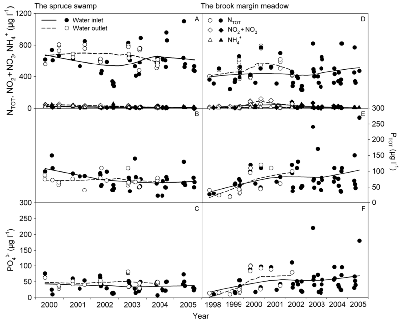
Fig. 7. Concentrations of N_{\text{TOT}} , \text{NO}_3 + \text{NO}_2 , \text{NH}_4^+ (A and D), P_{\text{TOT}} (B and E) and \text{PO}_4^{3-} (C and F) in the water inlet and outlet in the spruce swamp and the brook margin meadow.
