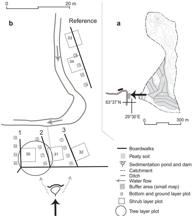
Fig. 2. Map of the brook-margin meadow study area. — a: Catchment — b: Overland flow buffer.
