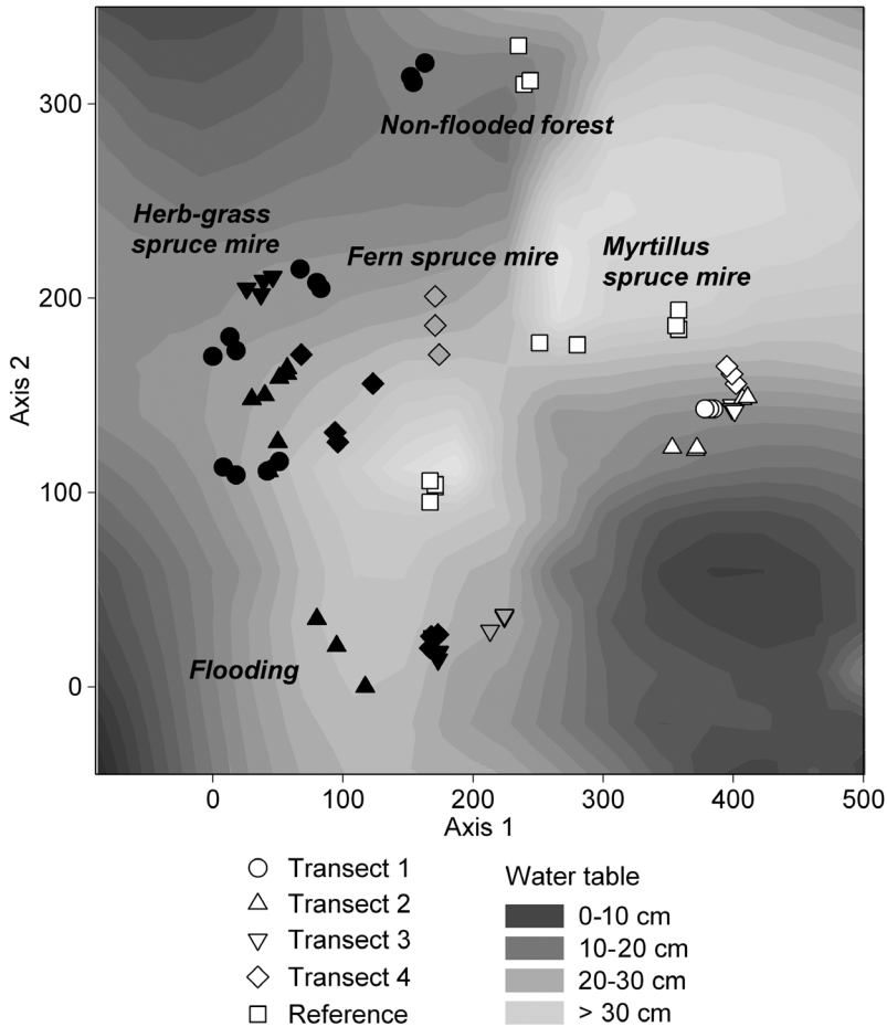
Fig. 3. DCA analysis of the spruce swamp with spatially smoothed average summer 2005 water table level for vegetation plots. Black symbols describe the flooded end, white symbols the non-flooded end of the buffer or reference, and gray symbols the vegetation plots with occasional flooding.
