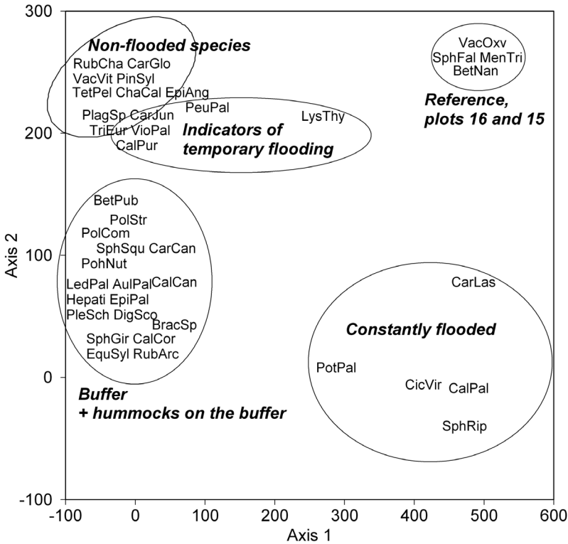
Fig. 6. DCA analysis for species on the brook margin meadow. Abbreviations of species were constructed by taking three first letters from both words of the species names (see Appendix 2).
