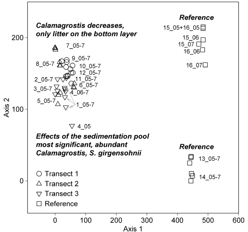
Fig. 5. DCA analysis for vegetation plots on the brook margin meadow. The numbers refer to vegetation plots (1–16) and years (2005–2007).
