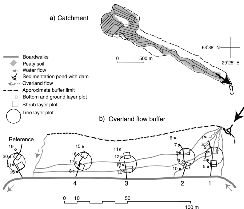
Fig. 1. Map of the spruce swamp study area.
