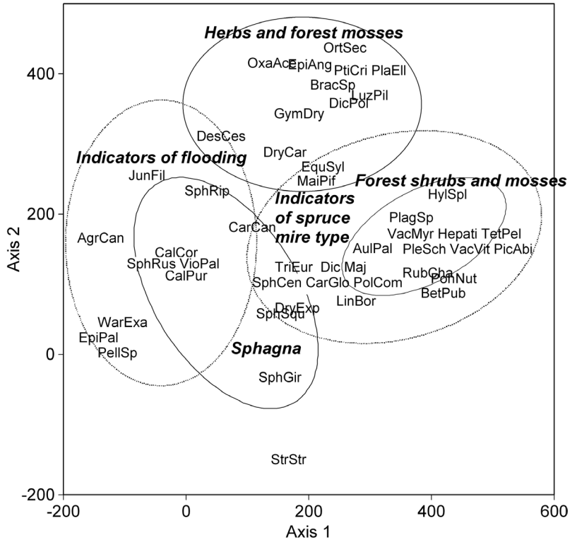
Fig. 4. DCA analysis for the species on the spruce swamp. The abbreviations of species were constructed by taking three first letters from both words of the species names (see Appendix 1).
