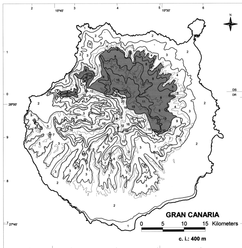
Fig. 5. Bioclimatic belts of Gran Canaria. Grey areas indicate territories with trade-wind clouds, including lower overcast areas below mist level. Numbers refer to Table 5.
