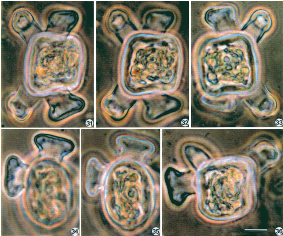
Figs. 31–36. Cosmarium taxillus var. taxillus , conjugation and zygospore formation. — 31 and 32 : Conjugating cells and zygospore in two different foci. — 33 : The same cell rotated 180 degrees. — 34 and 35 : The same cell rotated 45 degrees. — 36 : The same cell rotated 90 degrees relative to Figs. 31–35 . Scale bar = 10 \mu m.
